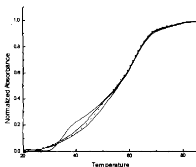
Figure 1: UV-melting curves for triplexes (a): 7*11:12, (b) 9*11:12, (c) 8*11:12 and (d) 10*11:12
